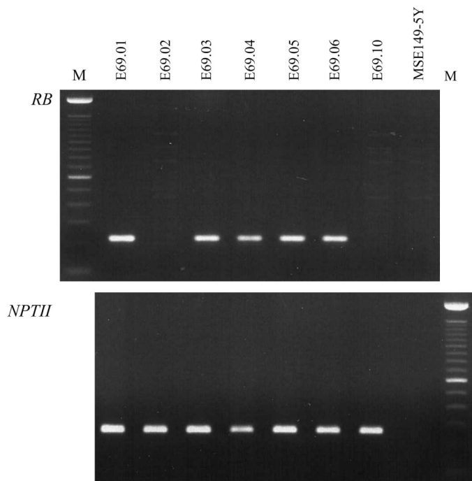
Fig. 2. PCR amplification of RB and NPTII fragments from total potato DNA. The expected RB fragment is 213 bp. Lanes E69.01, E69.02, E69.03, E69.04, E69.05, E69.06, and E69.10 are putative transformants; lane MSE149-5Y, untransformed control; lane M, 100-bp DNA ladder.
