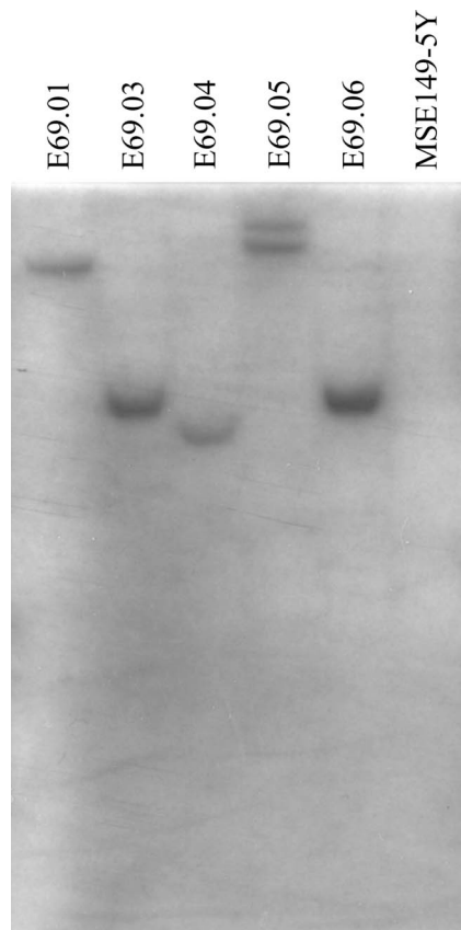
Fig. 3. Southern hybridization of Bam HI-digested total potato DNA with NPTII 700-bp fragment, 5-d exposure. Lanes E69.01, E69.03, E69.04, E69.05, and E69.06 are putative transformants; lane MSE149-5Y, untransformed control.
