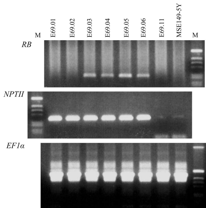
Fig. 4. Reverse-transcribed PCR of RB , NPTII , and EF1α . Expected fragments of RB , NPTII , and EF1α are 213, 267, and 400 bp, respectively. Lanes E69.01, E69.02, E69.03, E69.04, E69.05, E69.06, and E69.11 are putative potato transformants; lane MSE149-5Y, untransformed potato control; lane M, 1-kb DNA ladder.
