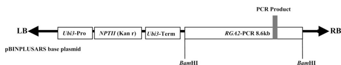
Fig. 1. T-DNA region of pSPUD69. RGA2-PCR indicates the 8.59-kb Bam HI fragment containing the RB gene ligated into the pBINPLUSARS base plasmid. This construct includes the NPTII gene for kanamycin resistance controlled by the ubiquitin ( Ubi3 ) promoter (Pro) and terminator (Term). Natural promoter (2503-bp upstream) and termination sequences (2477-bp downstream) were used for RB . The region in the T-DNA where the RB primers anneal is designated by “PCR Product.”
